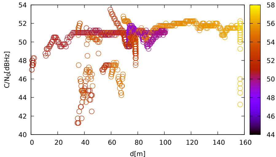
C/N 0 vs distance (JavadLSA at C 2 for E09 at L5)
