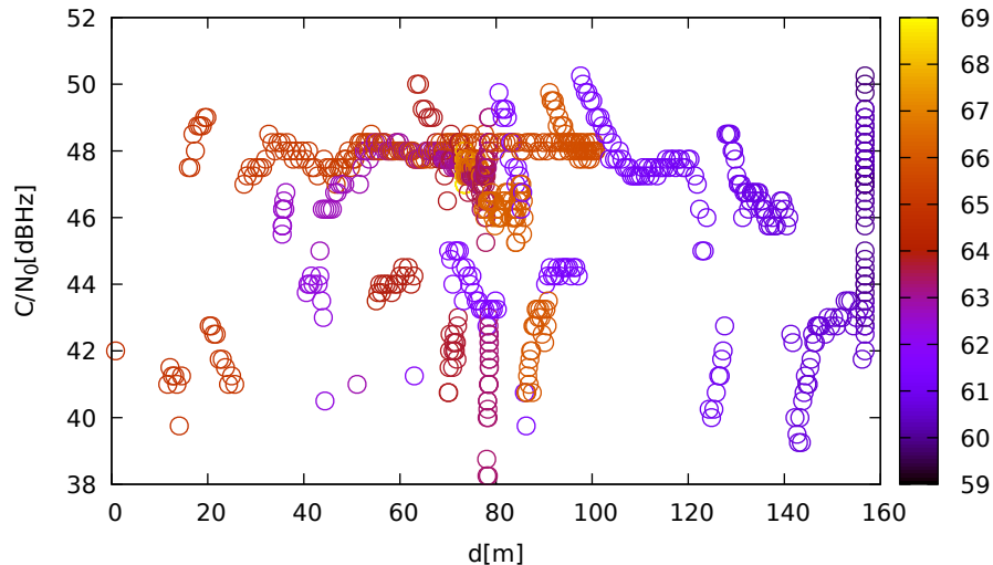
C/N 0 vs distance (JavadLSA at C 2 for E11 at L5)
