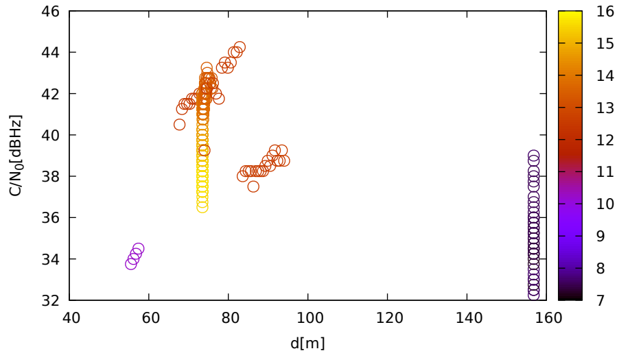
C/N 0 vs distance (JavadLSA at C 2 for E12 at L5)
