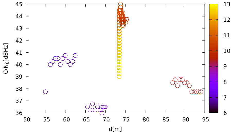
C/N 0 vs distance (JavadLSA at C 2 for E19 at L5)
