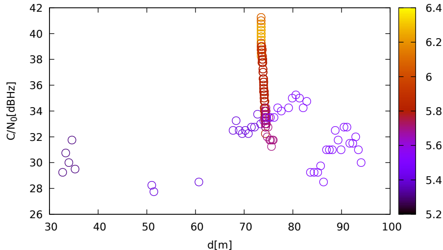
C/N 0 vs distance (JavadLSA at C 2 for E30 at L5)
