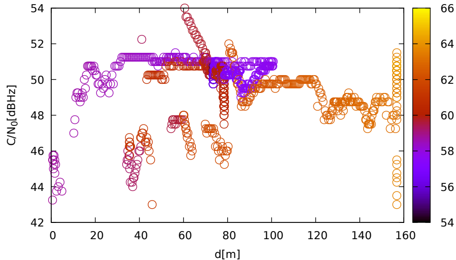
C/N 0 vs distance (JavadLSA at C 2 for E36 at L5)
