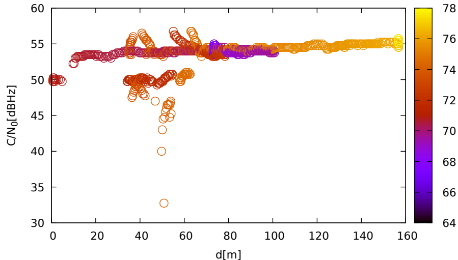
C/N 0 vs distance (JavadLSA at C 2 for G01 at L5)
