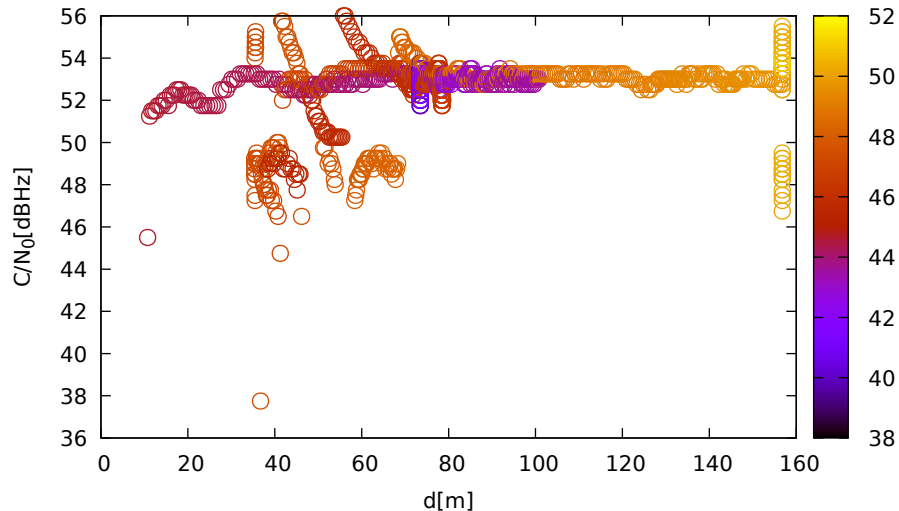
C/N 0 vs distance (JavadLSA at C 2 for G03 at L5)
