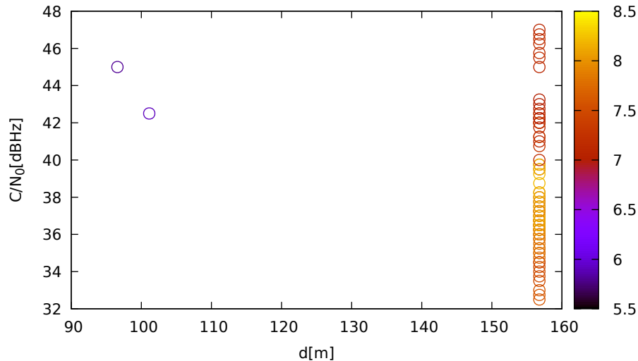
C/N 0 vs distance (JavadLSA at C 2 for G04 at L5)
