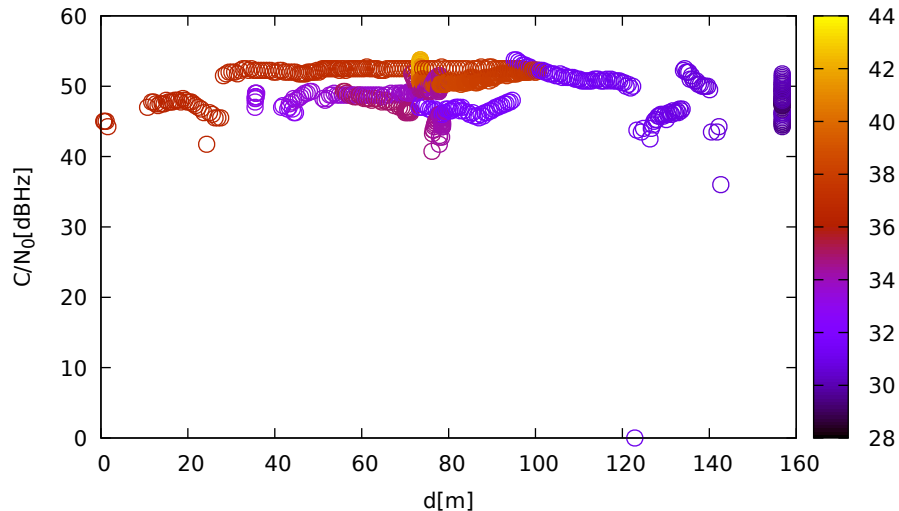
C/N 0 vs distance (JavadLSA at C 2 for G08 at L5)
