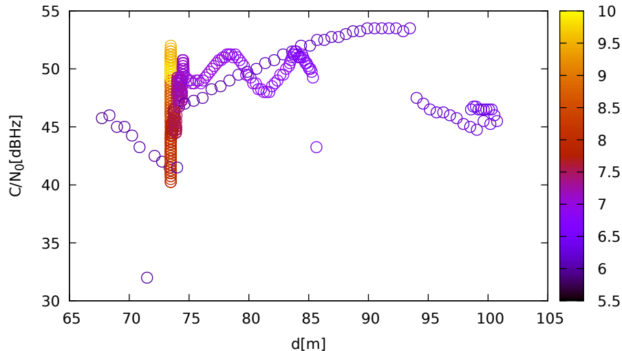
C/N 0 vs distance (JavadLSA at C 2 for G10 at L5)
