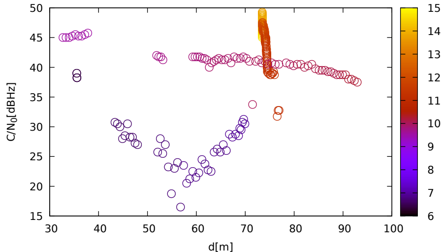
C/N 0 vs distance (JavadLSA at C 2 for G27 at L5)
