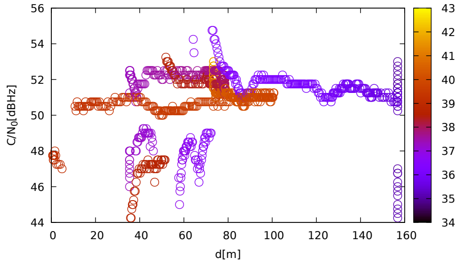
C/N 0 vs distance (JavadLSA at C 2 for G32 at L5)
