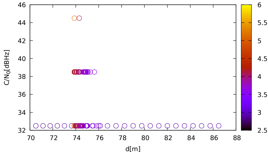
C/N 0 vs distance (LeicaGS15 at C 2 for E02 at L5)
