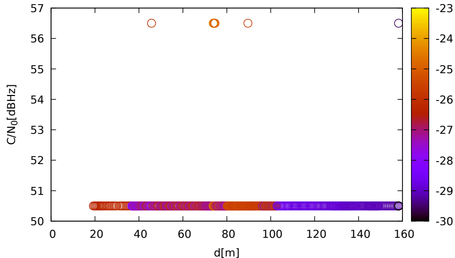
C/N 0 vs distance (LeicaGS15 at C 2 for E04 at L5)
