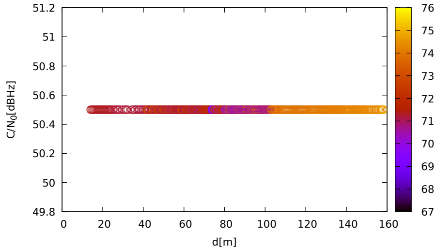
C/N 0 vs distance (LeicaGS15 at C 2 for E09 at L5)
