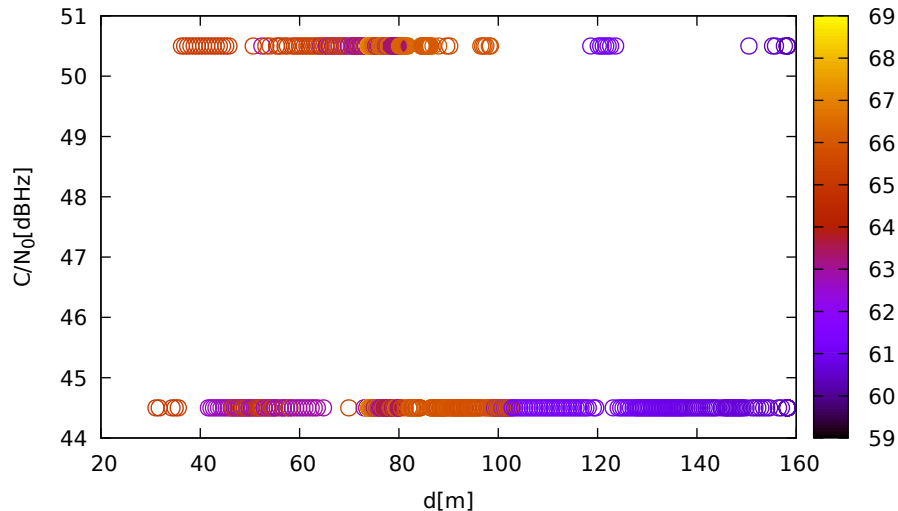
C/N 0 vs distance (LeicaGS15 at C 2 for E11 at L5)
