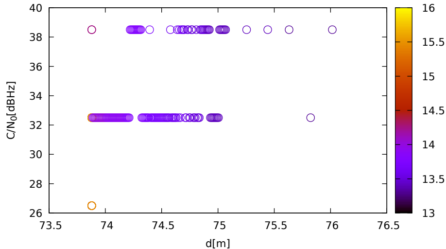
C/N 0 vs distance (LeicaGS15 at C 2 for E12 at L5)
