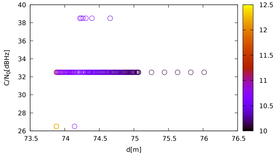
C/N 0 vs distance (LeicaGS15 at C 2 for E19 at L5)
