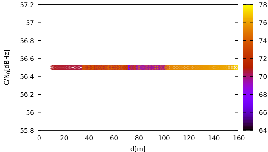
C/N 0 vs distance (LeicaGS15 at C 2 for G01 at L5)
