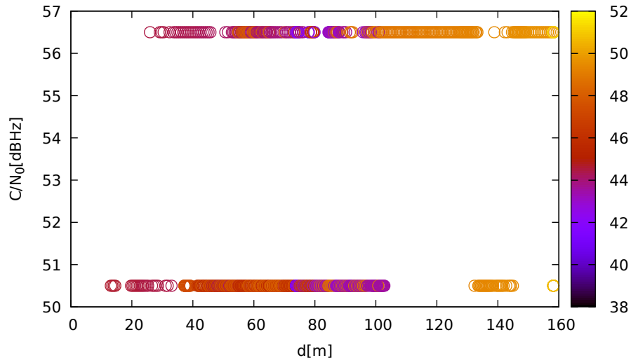
C/N 0 vs distance (LeicaGS15 at C 2 for G03 at L5)
