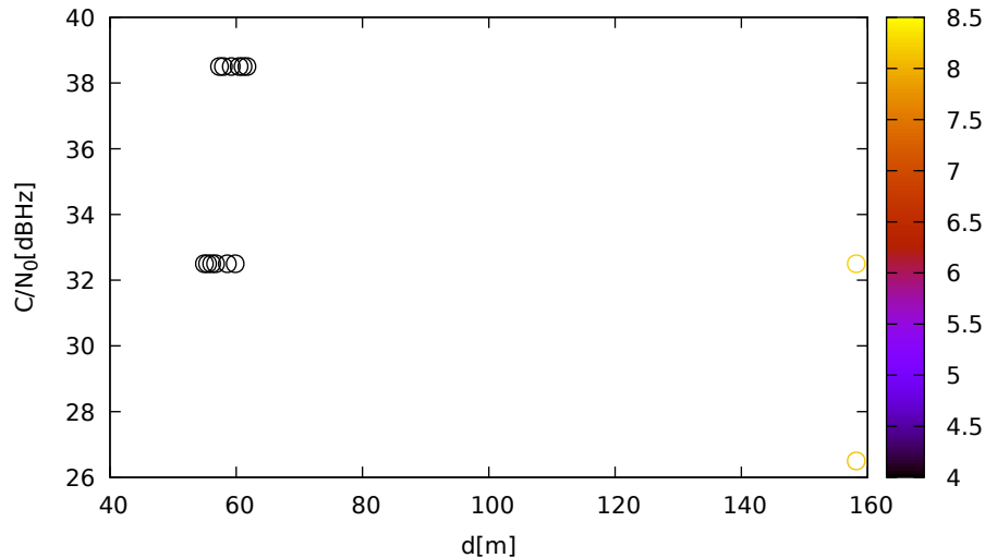
C/N 0 vs distance (LeicaGS15 at C 2 for G04 at L5)
