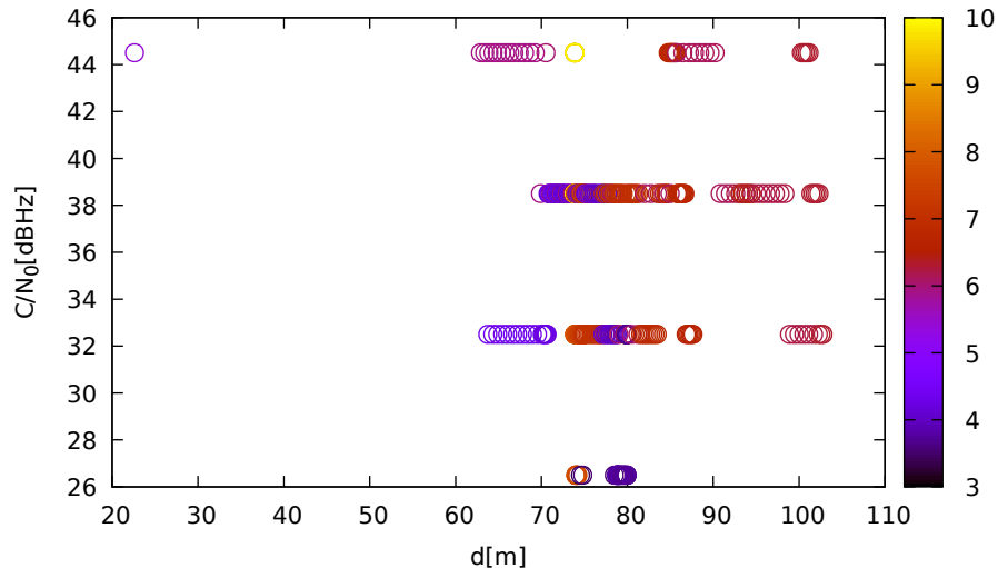
C/N 0 vs distance (LeicaGS15 at C 2 for G10 at L5)
