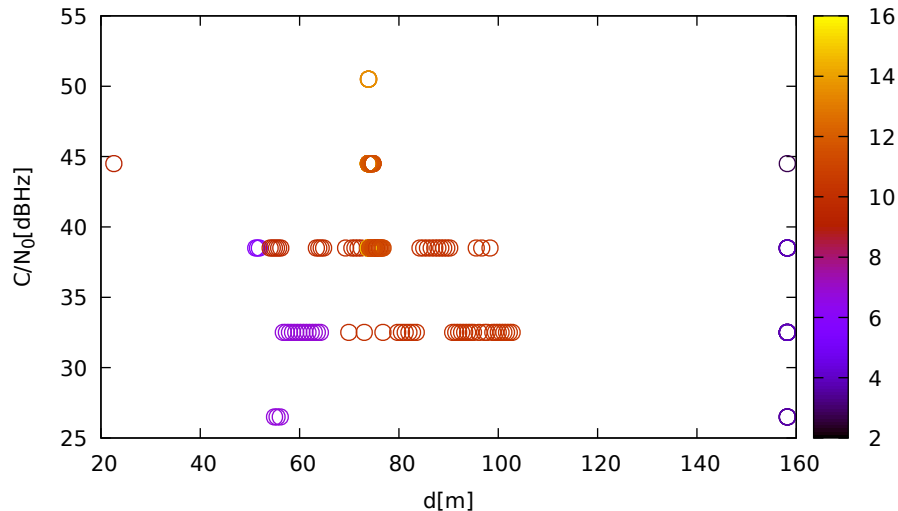
C/N 0 vs distance (LeicaGS15 at C 2 for G27 at L5)
