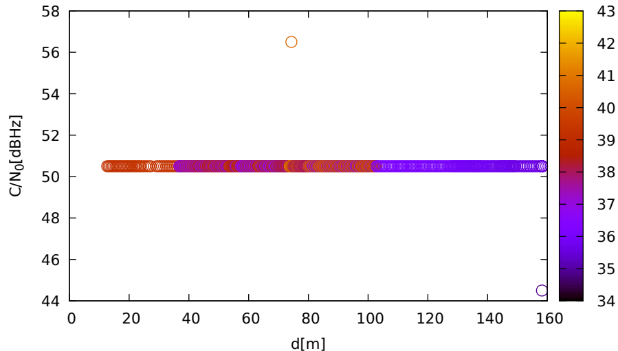
C/N 0 vs distance (LeicaGS15 at C 2 for G32 at L5)
