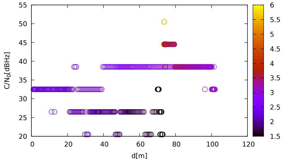
C/N 0 vs distance (LeicaGS18 at C 2 for E02 at L5)
