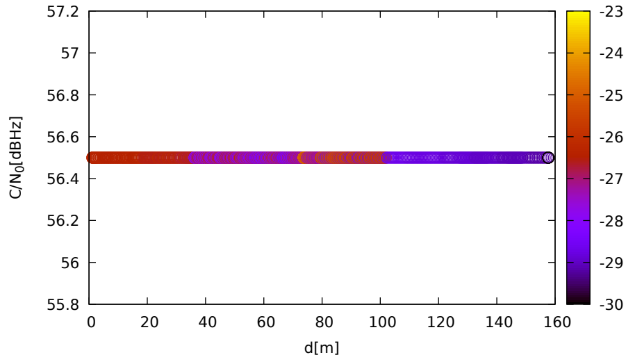
C/N 0 vs distance (LeicaGS18 at C 2 for E04 at L5)
