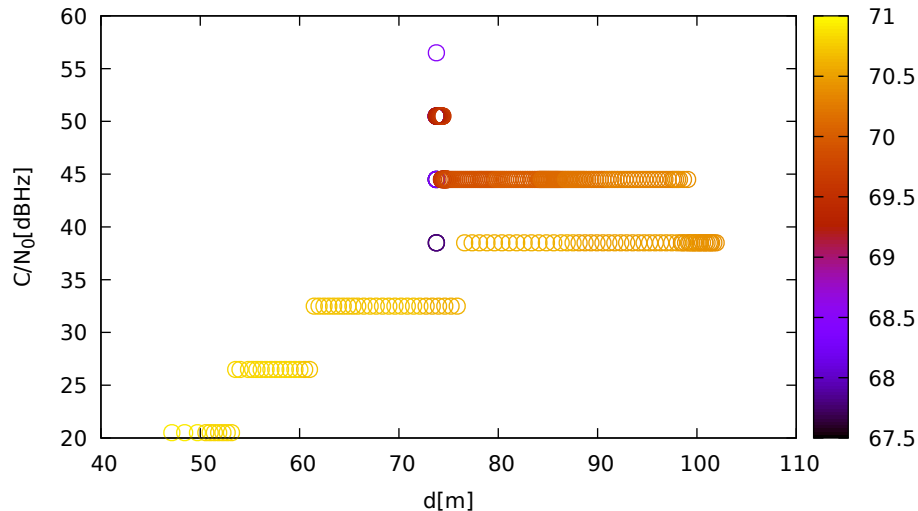
C/N 0 vs distance (LeicaGS18 at C 2 for E05 at L5)
