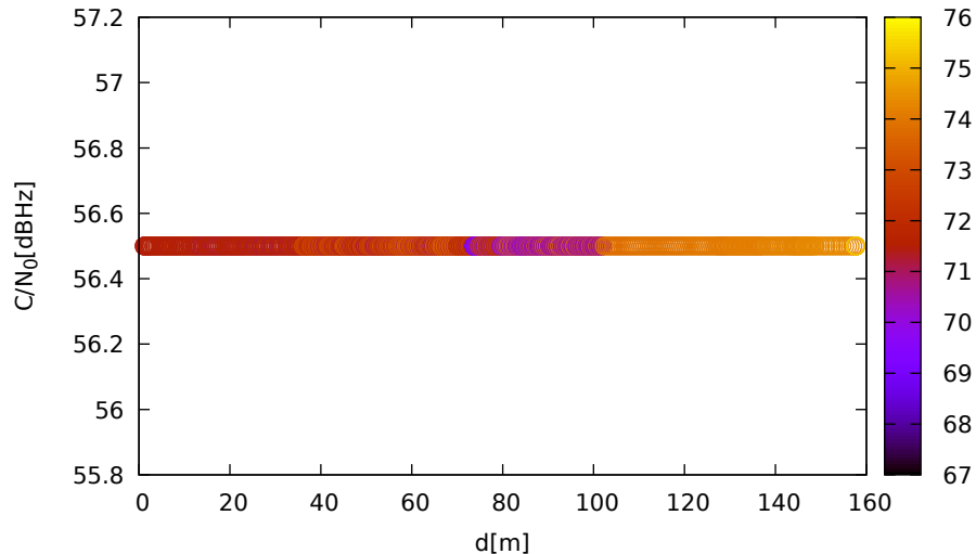
C/N 0 vs distance (LeicaGS18 at C 2 for E09 at L5)
