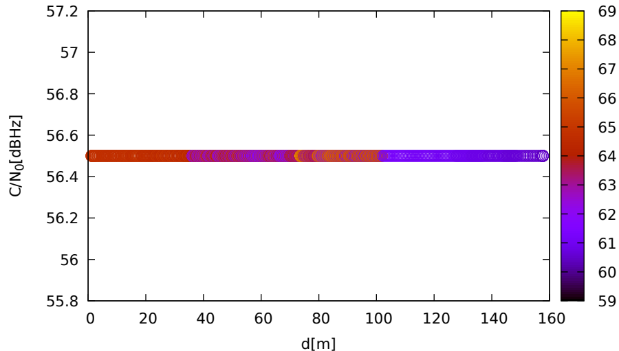
C/N 0 vs distance (LeicaGS18 at C 2 for E11 at L5)
