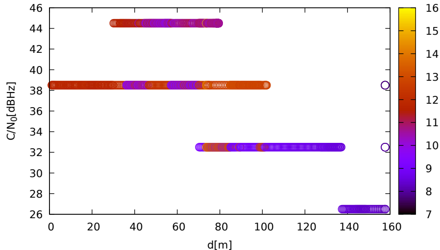
C/N 0 vs distance (LeicaGS18 at C 2 for E12 at L5)
