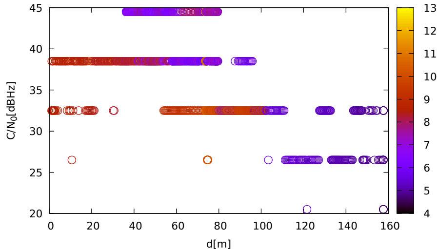
C/N 0 vs distance (LeicaGS18 at C 2 for E19 at L5)
