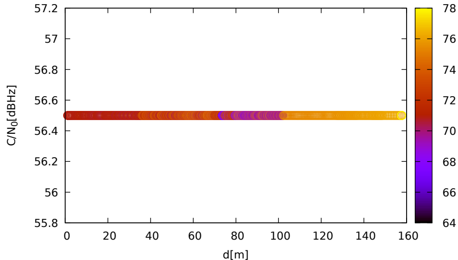
C/N 0 vs distance (LeicaGS18 at C 2 for G01 at L5)
