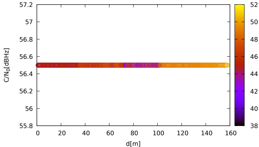
C/N 0 vs distance (LeicaGS18 at C 2 for G03 at L5)
