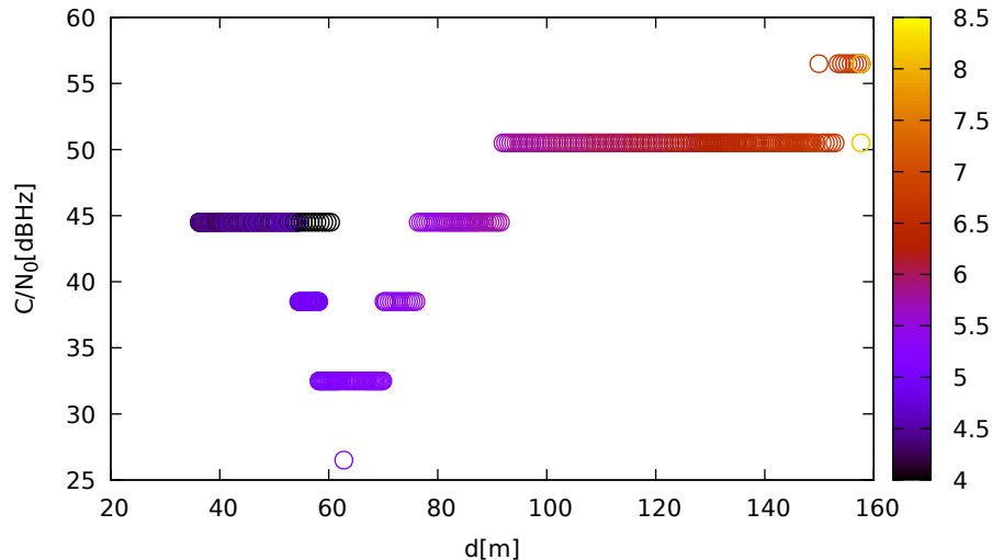
C/N 0 vs distance (LeicaGS18 at C 2 for G04 at L5)
