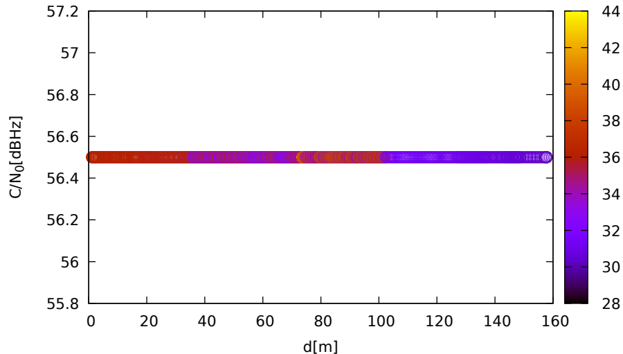
C/N 0 vs distance (LeicaGS18 at C 2 for G08 at L5)
