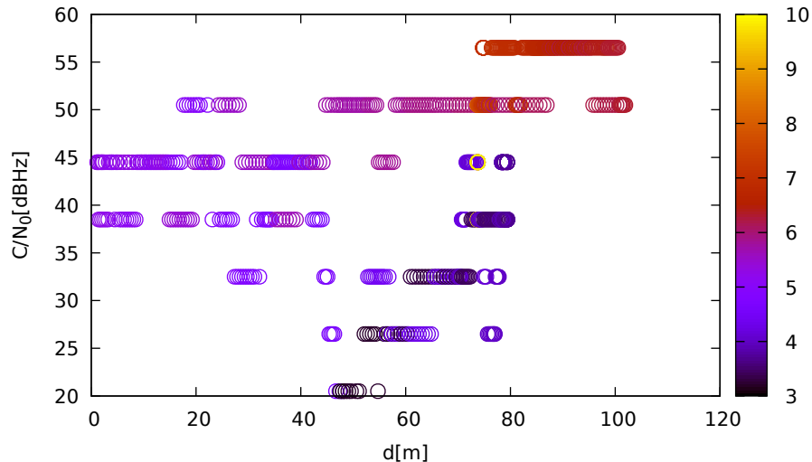
C/N 0 vs distance (LeicaGS18 at C 2 for G10 at L5)
