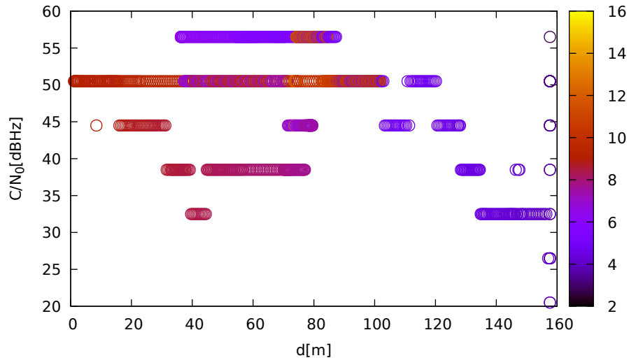
C/N 0 vs distance (LeicaGS18 at C 2 for G27 at L5)
