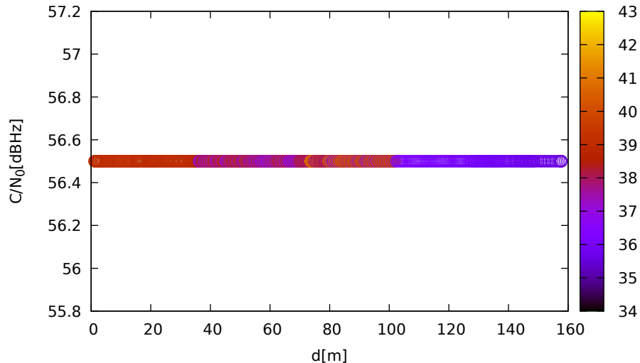
C/N 0 vs distance (LeicaGS18 at C 2 for G32 at L5)
