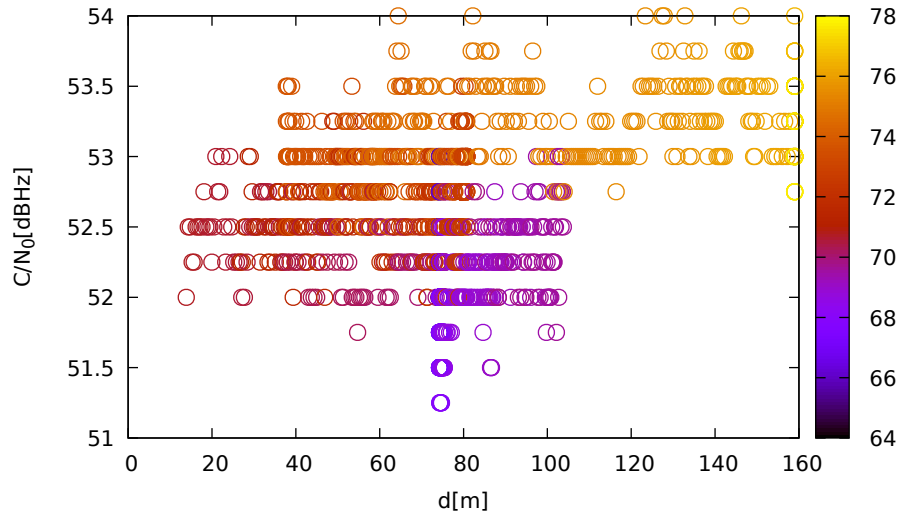
C/N 0 vs distance (TrimbleR10 at C 2 for G01 at L5)
