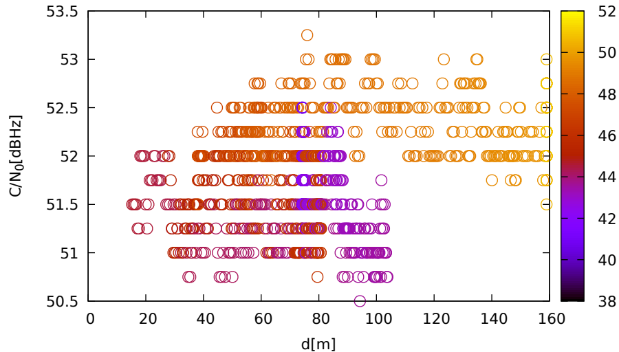
C/N 0 vs distance (TrimbleR10 at C 2 for G03 at L5)
