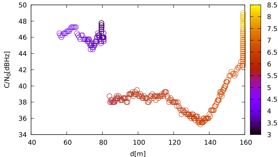
C/N 0 vs distance (TrimbleR10 at C 2 for G04 at L5)
