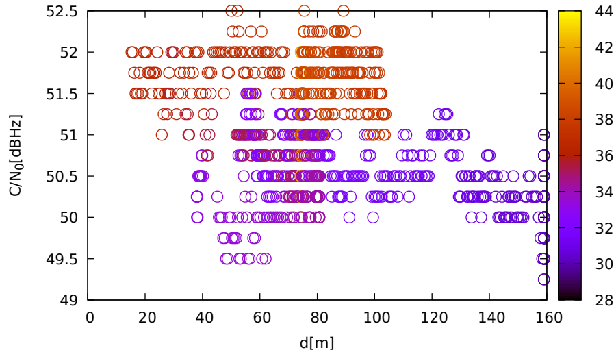
C/N 0 vs distance (TrimbleR10 at C 2 for G08 at L5)
