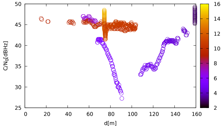
C/N 0 vs distance (TrimbleR10 at C 2 for G27 at L5)
