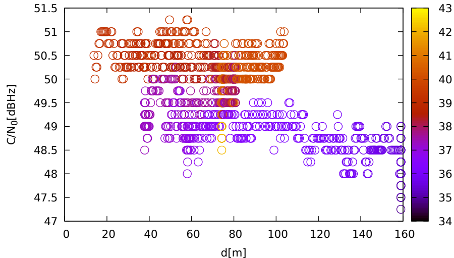
C/N 0 vs distance (TrimbleR10 at C 2 for G32 at L5)
