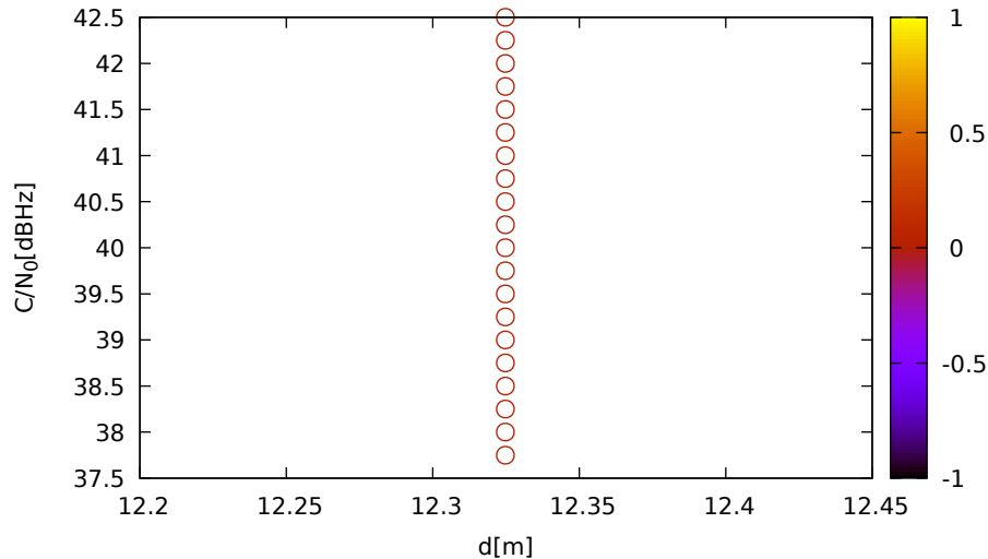
C/N 0 vs distance (JavadLSA at C 3 for E02 at L5)
