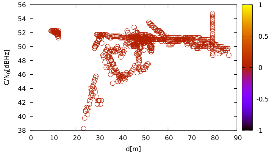
C/N 0 vs distance (JavadLSA at C 3 for E04 at L5)
