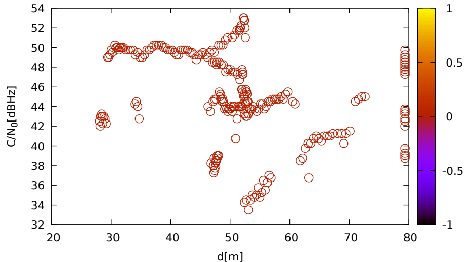
C/N 0 vs distance (JavadLSA at C 3 for E05 at L5)
