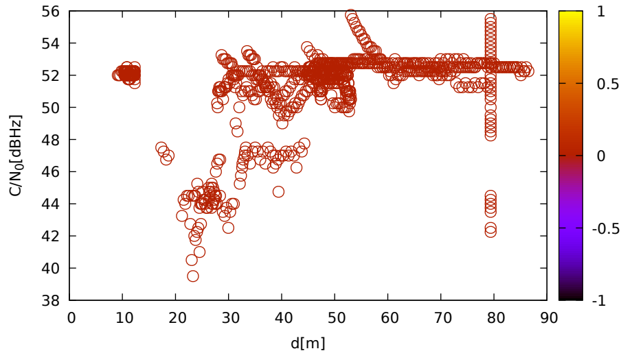
C/N 0 vs distance (JavadLSA at C 3 for E09 at L5)
