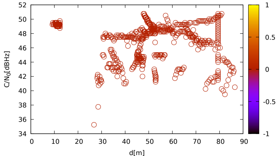
C/N 0 vs distance (JavadLSA at C 3 for E11 at L5)
